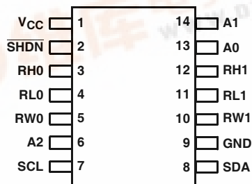
ISL22326WMVEP (14 LD TSSOP) TOP VIEW
