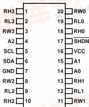
ISL22346WMVEP (20 LD TSSOP) TOP VIEW
