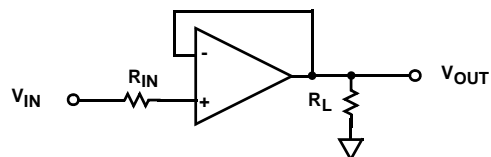
FIGURE 38. INPUT CURRENT LIMITING
