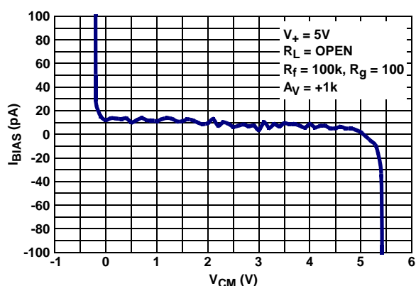
FIGURE 19. INPUT BIAS CURRENT vs COMMON MODE INPUT VOLTAGE
