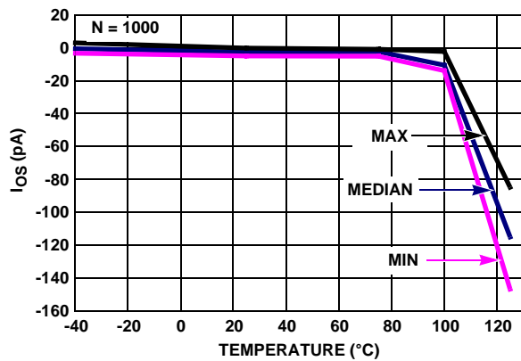
FIGURE 32. I_{OS} vs TEMPERATURE, V_+, V_- = \pm 2.5
