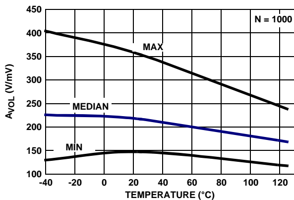
FIGURE 36. A_{VOL} vs TEMPERATURE, V_+, V_- = \pm 2.5V, V_O = -2V \text{ TO } +2V, R_L = 100k
