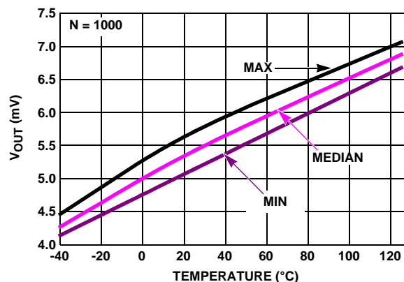
FIGURE 41. V_{OUT \text{ LOW}} vs TEMPERATURE, V_+, V_- = \pm 2.5V, R_L = 100k
