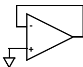
FIGURE 45. PREVENTING OSCILLATIONS IN UNUSED CHANNELS
