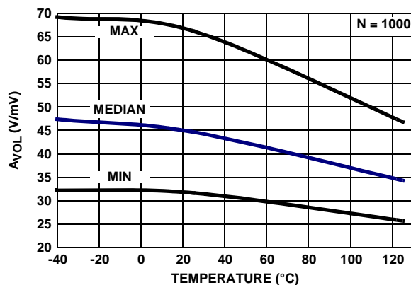
FIGURE 37. A_{VOL} vs TEMPERATURE, V_+, V_- = \pm 2.5V, V_O = -2V \text{ TO } +2V, R_L = 1k
