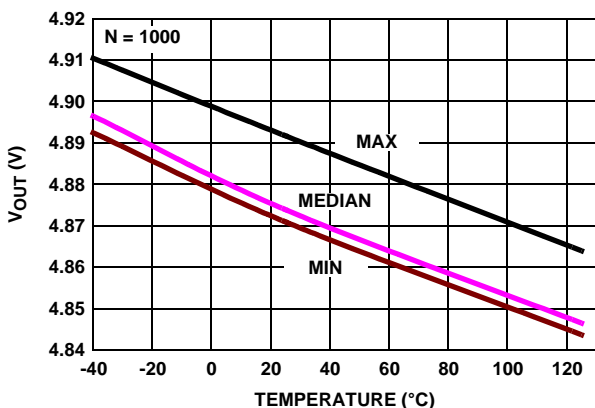
FIGURE 38. V_{OUT \text{ HIGH}} vs TEMPERATURE, V_+, V_- = \pm 2.5V, R_L = 1k
