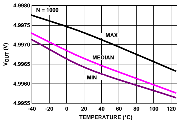
FIGURE 39. V_{OUT \text{ HIGH}} vs TEMPERATURE, V_+, V_- = \pm 2.5V, R_L = 100k
