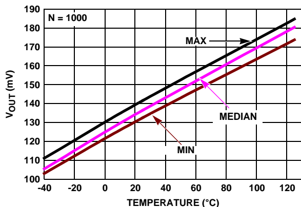
FIGURE 40. V_{OUT \text{ LOW}} vs TEMPERATURE, V_+, V_- = \pm 2.5V, R_L = 1k
