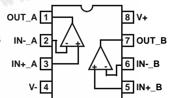
ISL28266 (8 LD SOIC) TOP VIEW
