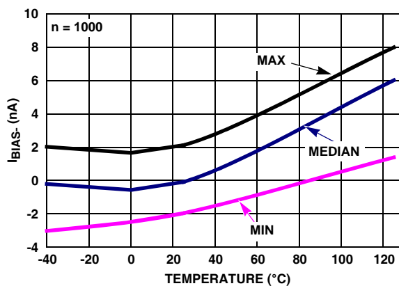
FIGURE 26. I_{BIAS-} vs TEMPERATURE, V_S = \pm 1.2V
