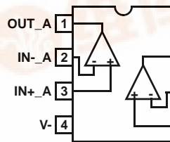
ISL28266 (8 LD MSOP) TOP VIEW
