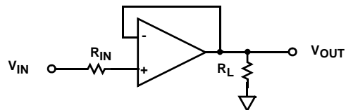
FIGURE 35. INPUT CURRENT LIMITING
