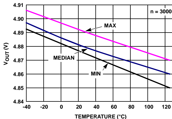
FIGURE 30. ISL28272 V_{OUT} HIGH vs TEMPERATURE R_L = 1k , V_S = \pm 2.5V
