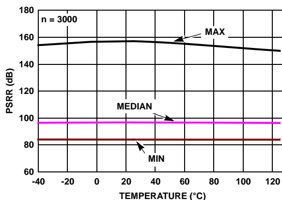
FIGURE 28. ISL28272 PSRR vs TEMPERATURE V_S = \pm 1.2V TO \pm 2.5V
