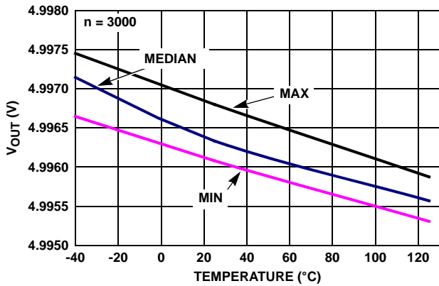
FIGURE 31. ISL28271 V_{OUT} HIGH vs TEMPERATURE R_L = 100k , V_S = \pm 2.5V
