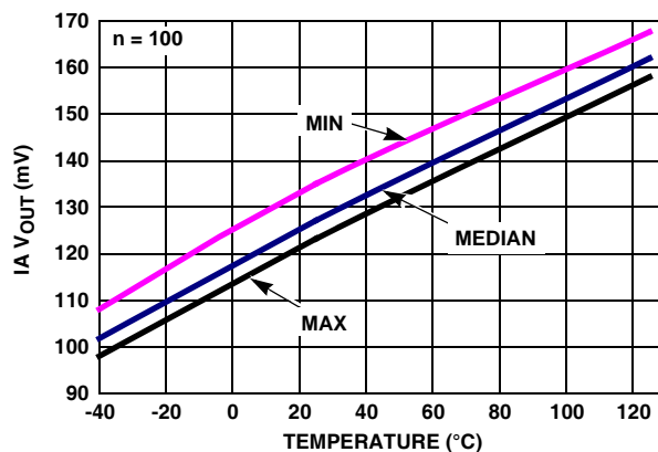
FIGURE 56. IA V_{OUT} LOW vs TEMPERATURE R_L = 1k . V_S = \pm 2.5V
