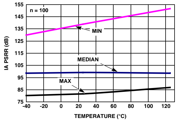
FIGURE 52. IA PSRR vs TEMPERATURE V_S = \pm 2.5V
