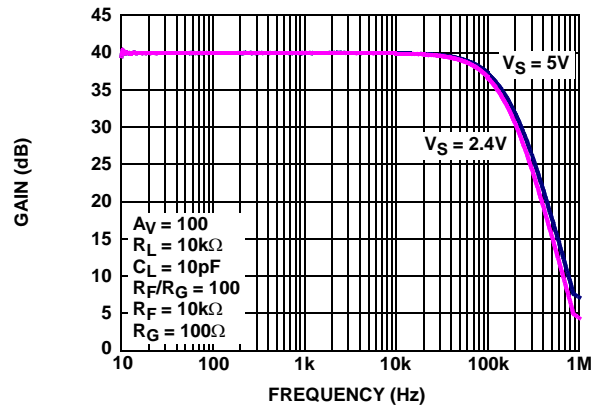
FIGURE 4. AMPLIFIER "A" (INAMP) FREQUENCY RESPONSE vs SUPPLY VOLTAGE
