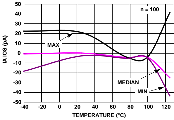
FIGURE 43. IA INPUT OFFSET CURRENT vs TEMPERATURE V_S = \pm 1.2V
