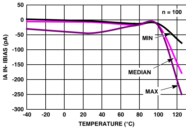
FIGURE 35. I BIAS (IA IN-) vs TEMPERATURE V_S = \pm 2.5V
