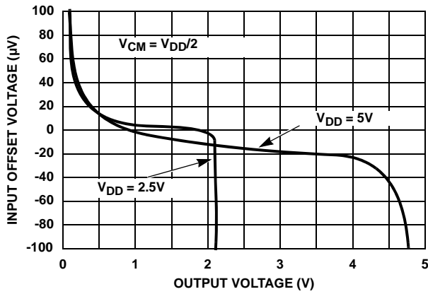
FIGURE 13. AMPLIFIER "B" (OP-AMP) INPUT OFFSET VOLTAGE vs OUTPUT VOLTAGE
