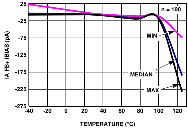
FIGURE 32. I BIAS (IA FB+) vs TEMPERATURE V_S = \pm 1.2V
