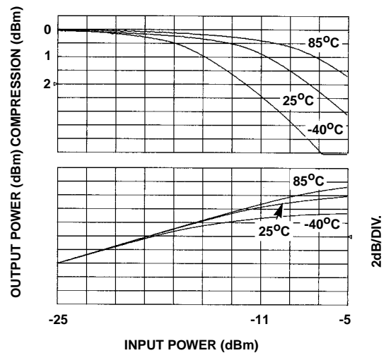
FIGURE 8. GAIN COMPRESSION OVER TEMPERATURE
