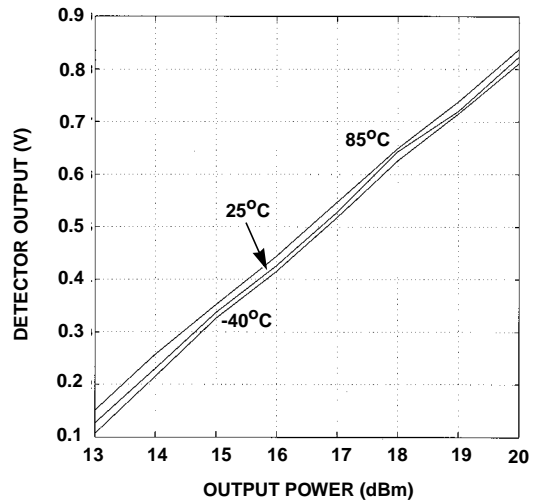
FIGURE 12. DETECTOR OUTPUT OVER TEMPERATURE
