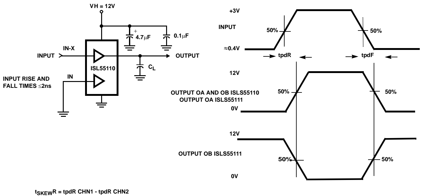
FIGURE 2. TEST CIRCUIT PROPAGATION TPD DELAY
