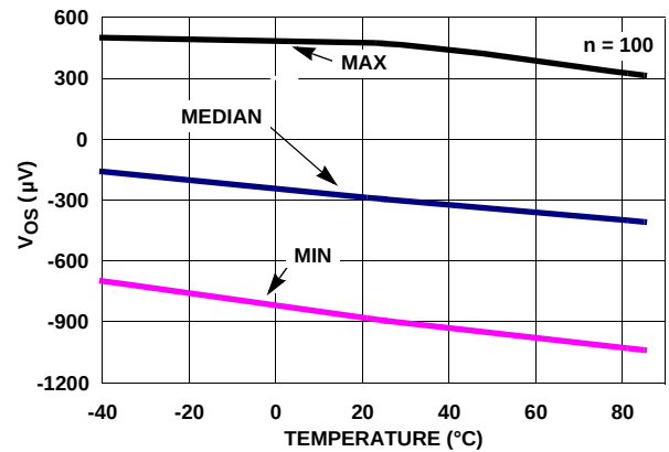
FIGURE 34. V_{I0} vs TEMPERATURE V_S = \pm 1.5V
