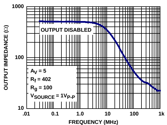
FIGURE 12. DISABLED OUTPUT IMPEDANCE vs FREQUENCY
