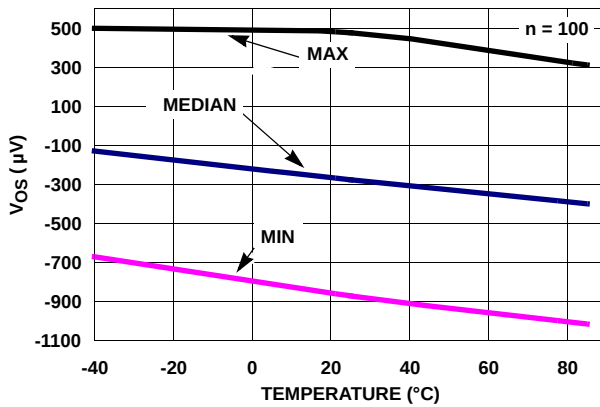
FIGURE 33. V_{I0} vs TEMPERATURE V_S = \pm 2.5V
