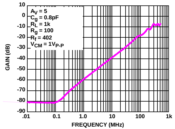
FIGURE 14. CMRR vs FREQUENCY
