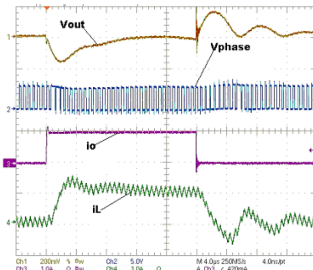
FIGURE 9. LOAD TRANSIENT ( V_{IN} = 3.6V ; V_O = 1.6V ; I_O = 0A \sim 1A )
