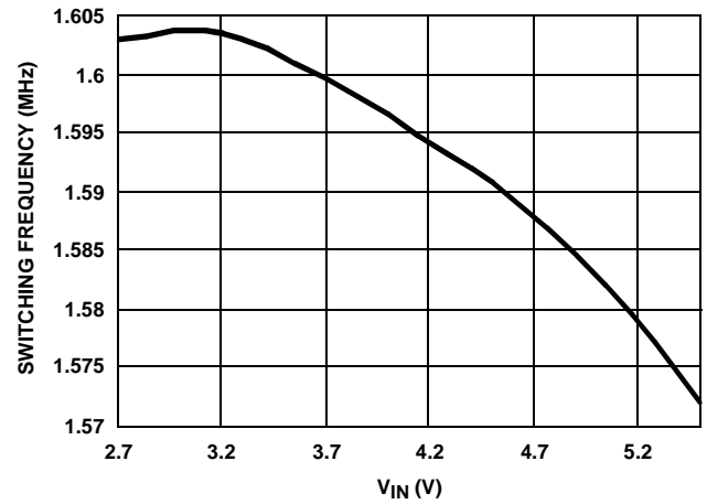
FIGURE 4. SWITCHING FREQUENCY vs V_{IN}
