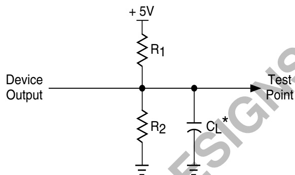
Figure 2. Test Load
