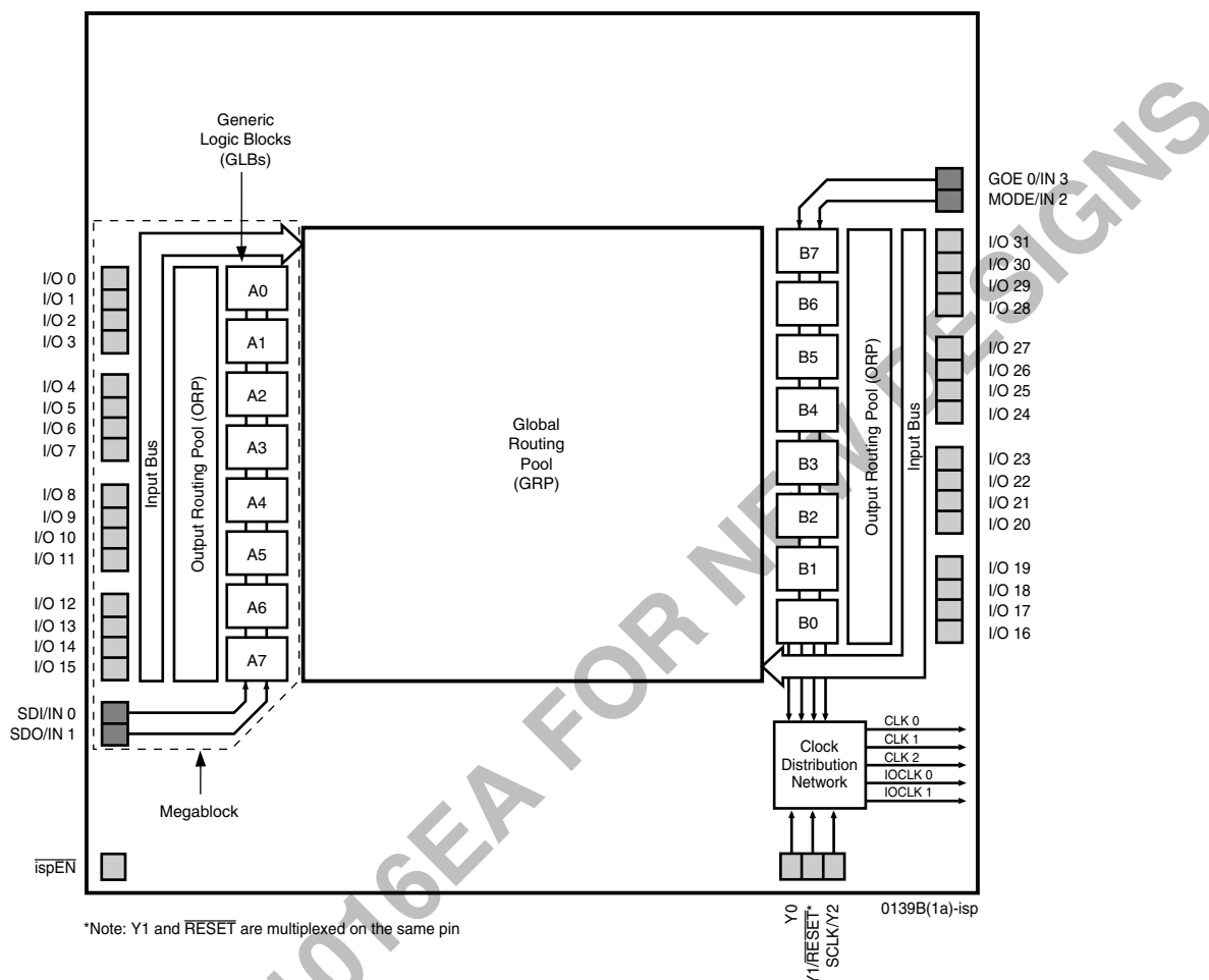
Figure 1. ispLSI 1016E Functional Block Diagram
