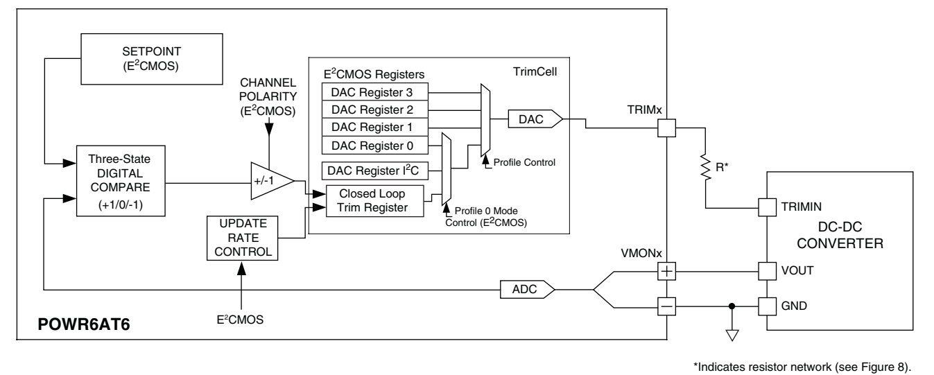
Figure 10. Digital Closed Loop Trim Operation
