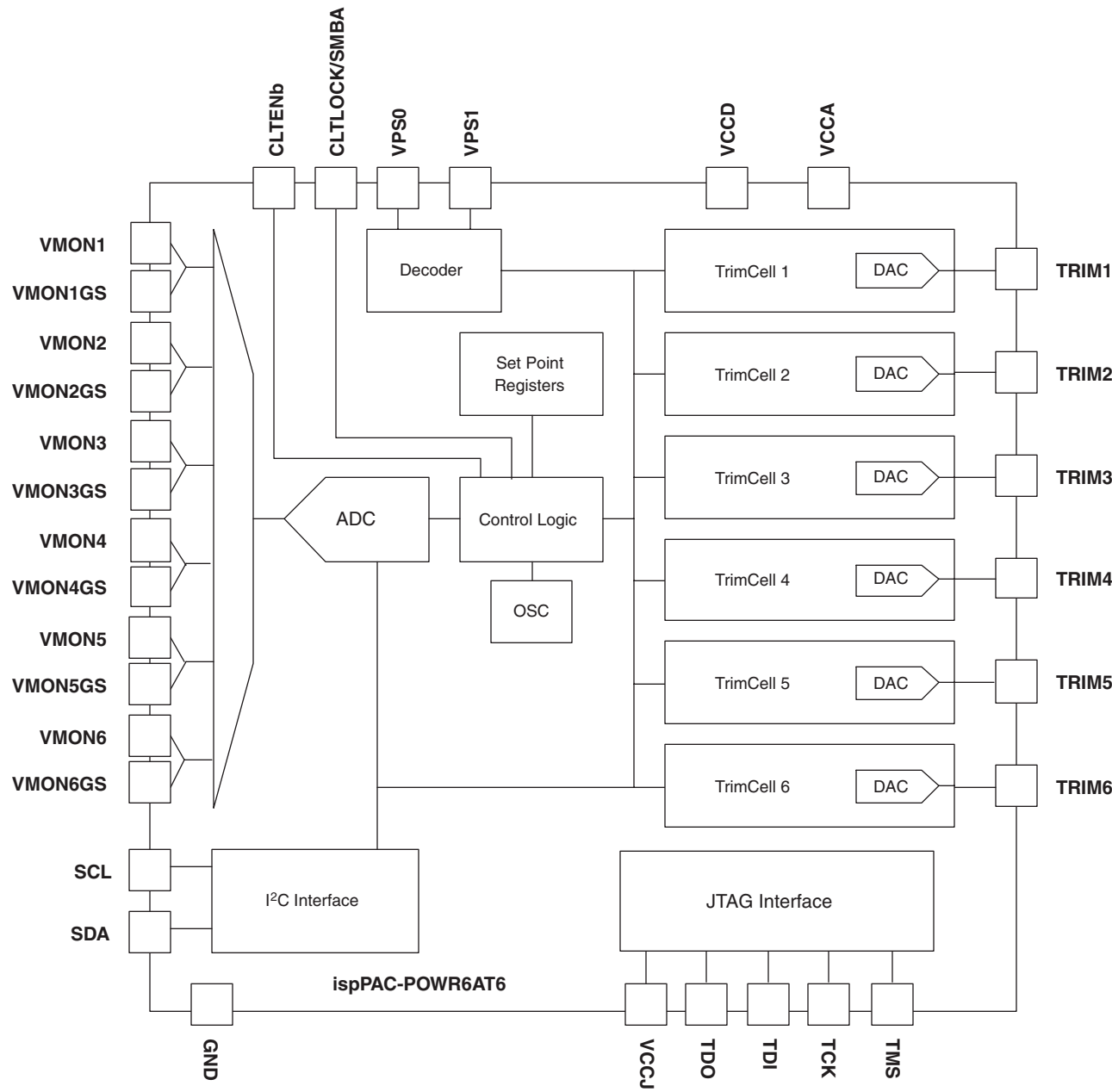
Figure 1. ispPAC-POWR6AT6 Block Diagram
