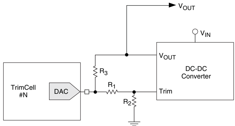
Figure 8. TrimCell Driving a Typical DC-DC Converter
