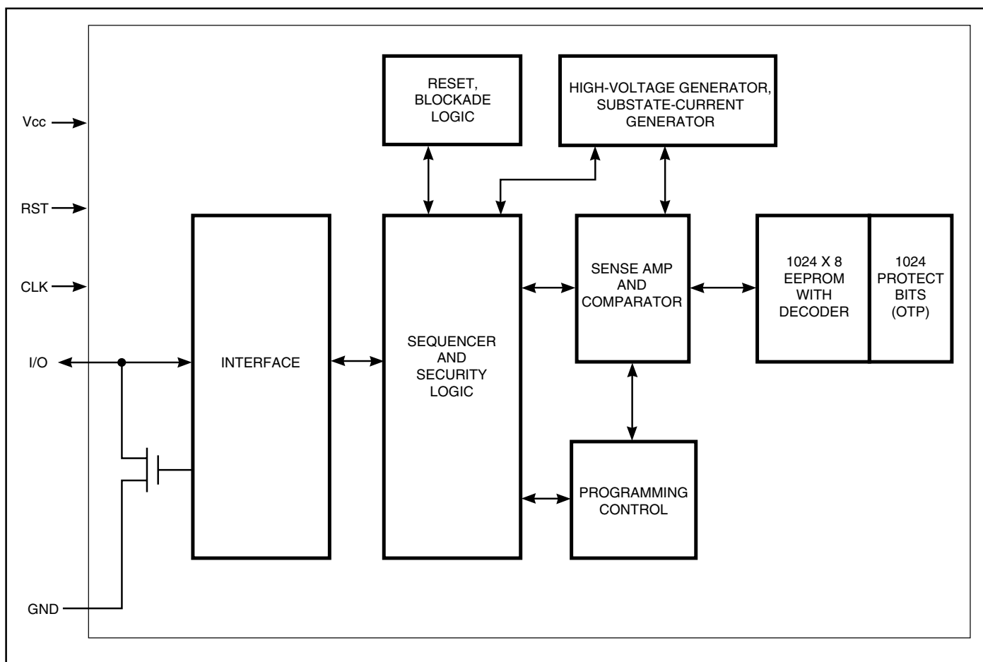
Figure 1. Block Diagram
