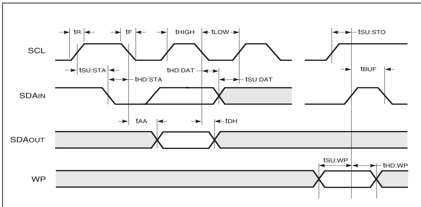
Figure 11. Bus Timing
