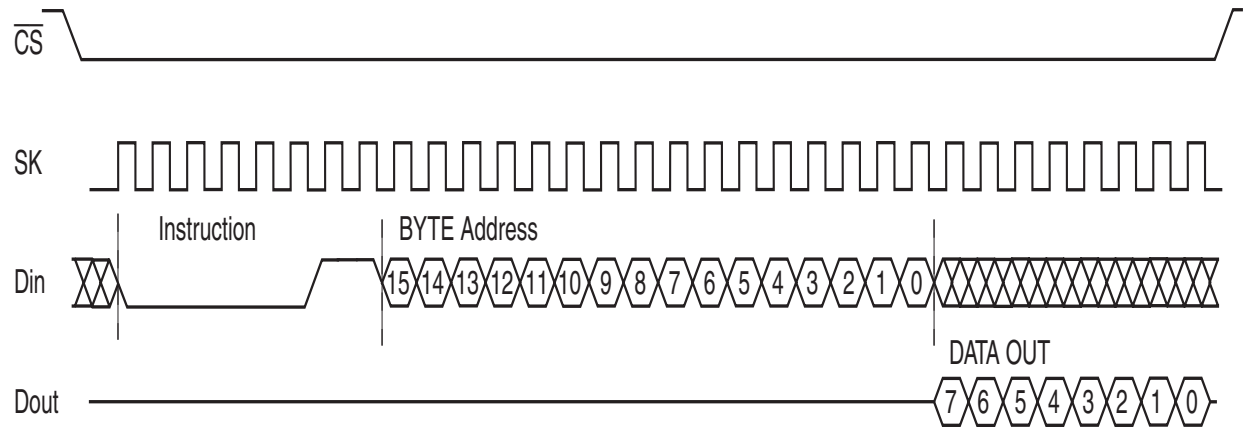
Figure 6. READ Timing
