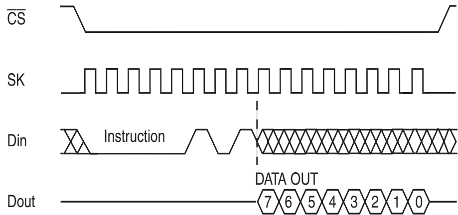
Figure 4. RDSR Timing
