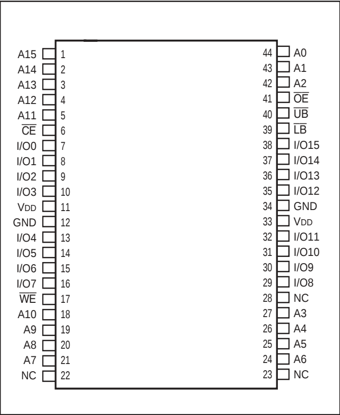
44-Pin TSOP-II
