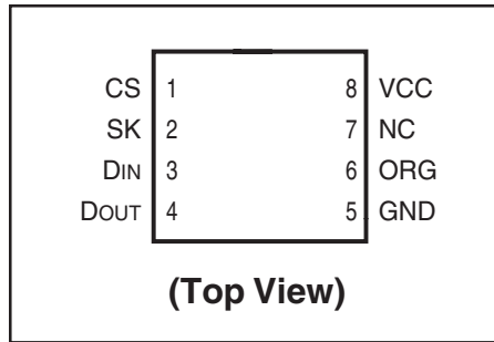
8-pad DFN
