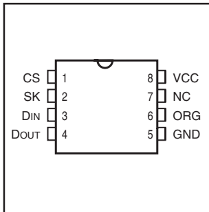
8-Pin DIP
