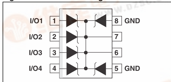
Figure 1. Functional diagram
