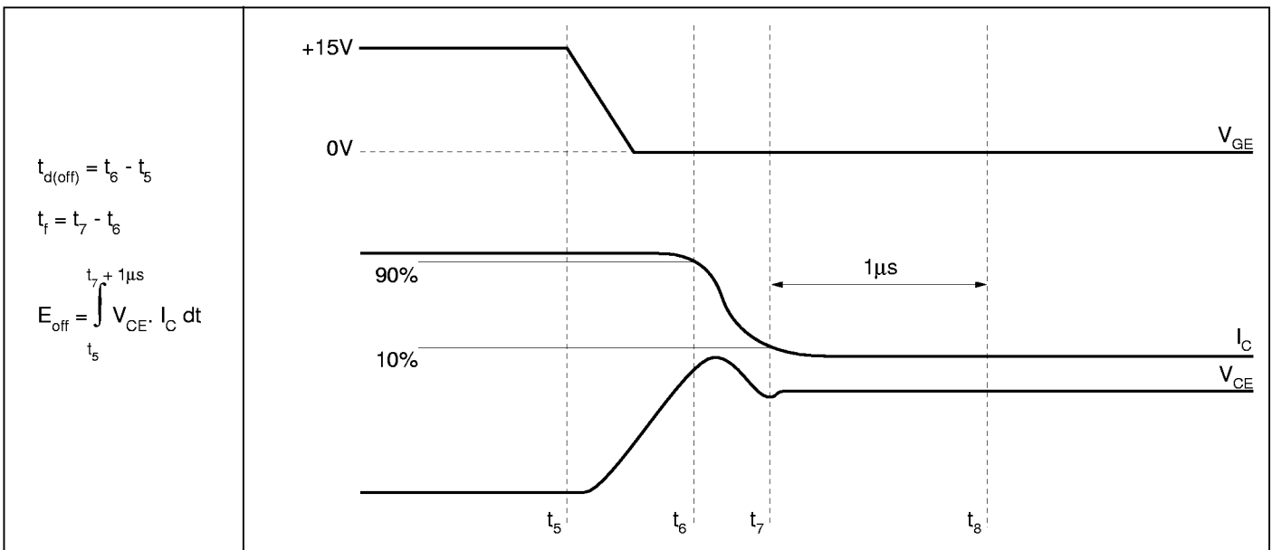
Fig.5 Turn-off characteristics
