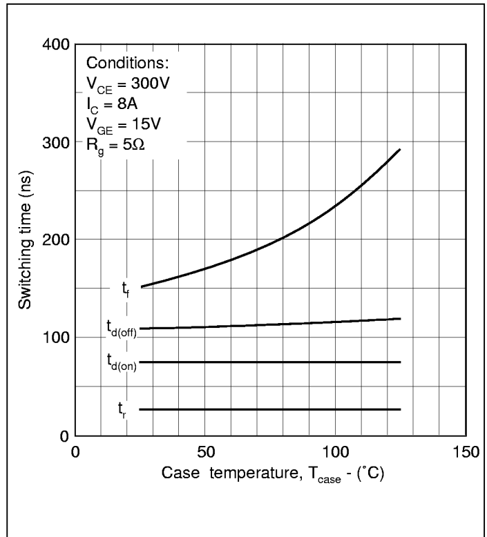
Fig.13 Typical switching time vs case temperature
