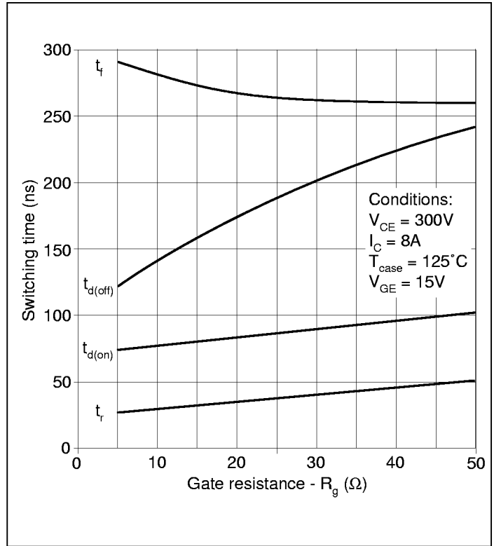
Fig.11 Typical switching times vs gate resistance
