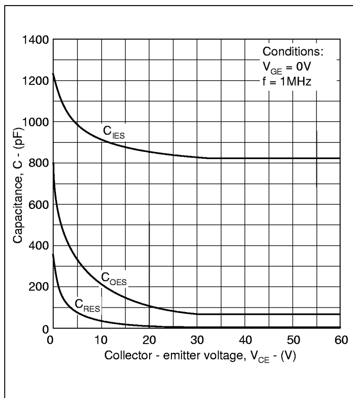
Fig.14 Typical capacitance
