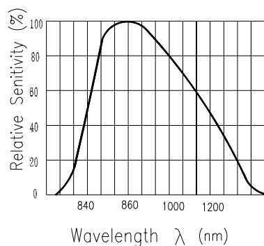
Fig.5 Spectral Sensitivity
