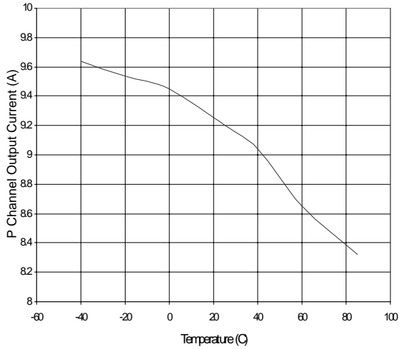
Fig. 21 P Channel Output Current vs. Temperature V_{CC}=18V, C_L=10nF
