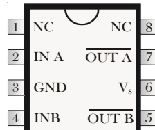
8 Lead PDIP (PI) 8 Pin SOIC (SI) IXDI404
