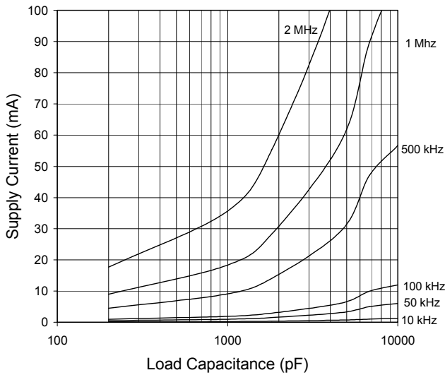
Fig. 15 Supply Current vs. Load Capacitance V cc = 18V
