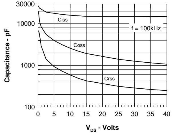
Fig.8 Capacitance Curves
