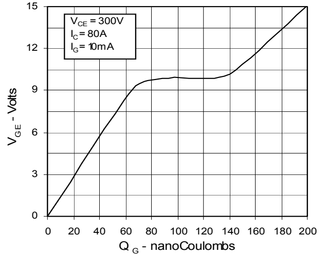
Fig. 14. Gate Charge
