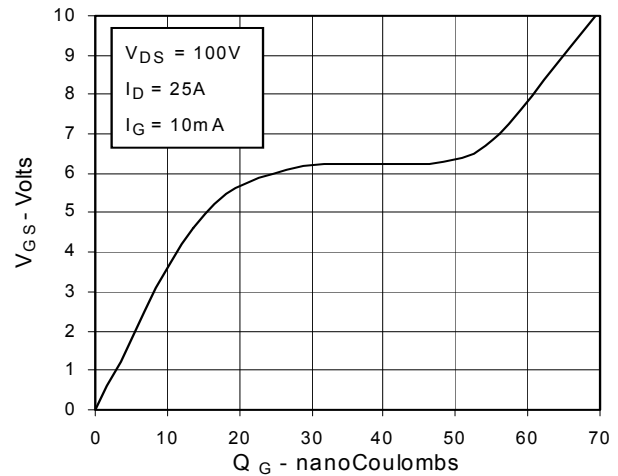
Fig. 10. Gate Charge
