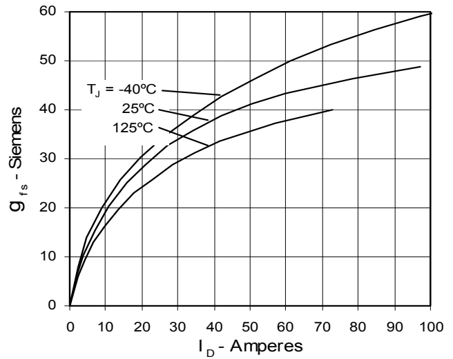
Fig. 8. Transconductance
