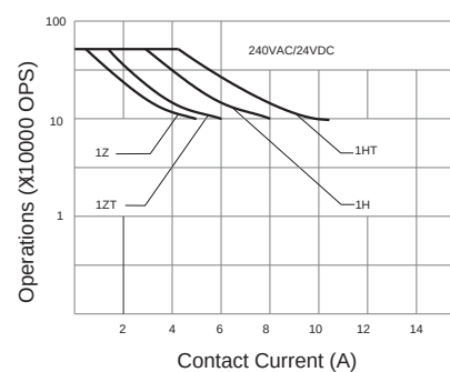
LIFE CURVE
