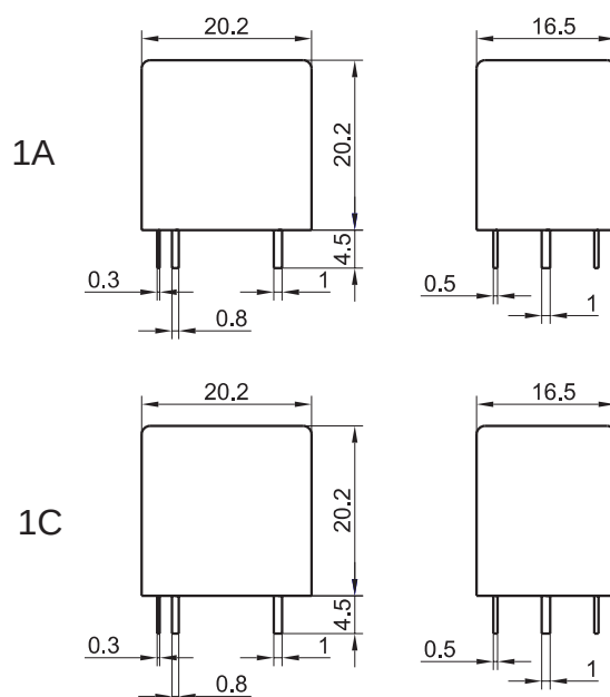
Outline Dimensions
