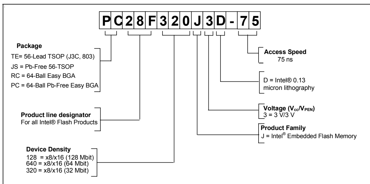
Figure 30: Decoder for Discrete Family (32, 64 and 128 Mbit)
