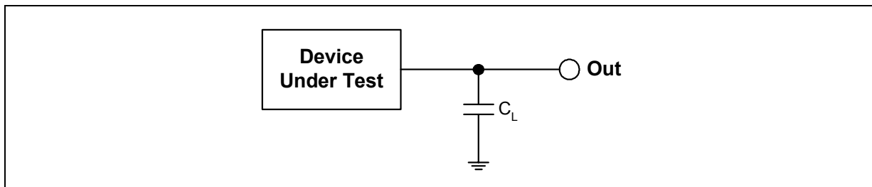
Figure 12: Transient Equivalent Testing Load Circuit
