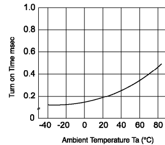
Fig.3 Turn on time vs. ambient temperature Load voltage 60V(DC) LED current: 5mA Continuous load current:400mA(DC)
