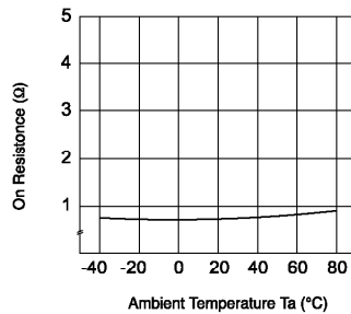
Fig.2 On resistance vs. ambient temperature Across terminals 3 and 4 pin LED current: 5mA Continuous load current:400mA(DC)
