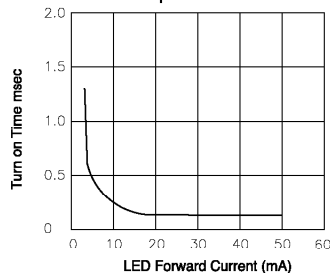
Fig.10 LED forward current vs. turn on time Across terminals 3 and 4 pin; Load voltage: 60V (DC) ; Continuous load current:400mA (DC); Ambient temperature: 25°C
