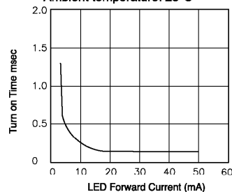
Fig.10 LED forward current vs. turn on time Across terminals 3 and 4 pin; Load voltage: 60V (DC) ; Continuous load current:200mA (DC); Ambient temperature: 25°C
