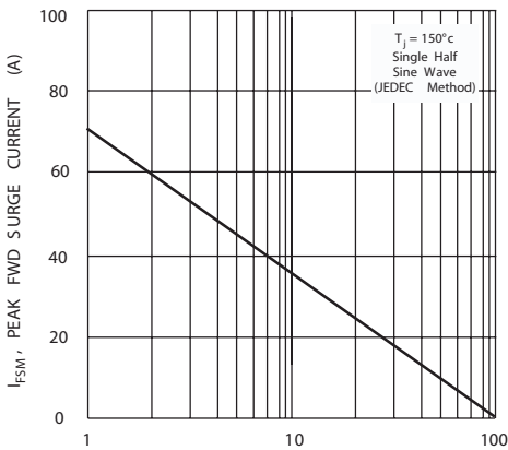
Fig. 3 Max Non-Repetitive Peak Fwd Surge Current
