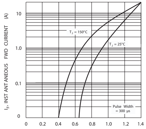
Fig. 2 Typical Fwd Characteristics
