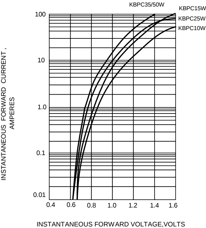
FIG.3-TYPICAL FORWARD CHARACTERISTICS
