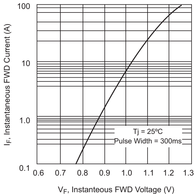
Fig. 2 Typical Forward Characteristics, per element
