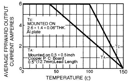
FIG. 2 - TYPICAL FORWARD OUTPUT DERATING CURVE
