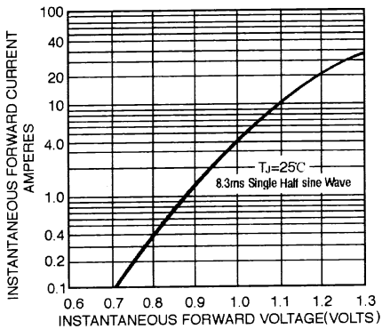
FIG. 3 - TYPICAL INSTANTANEOUS FORWARD CURRENT PER BRIDGE ELEMENT
