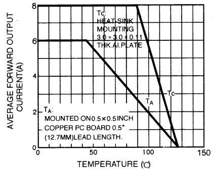
FIG. 2 - TYPICAL FORWARD OUTPUT CURRENT DERATING CURVE
