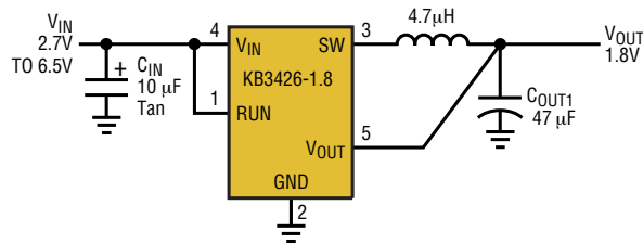
Single Li-Ion 1.8V/800mA Regulator for Low Output Ripple and Small Footprint
