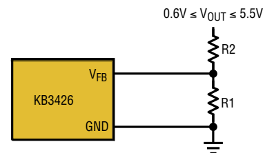
Figure 3. Setting the kB3426 Output Voltage
