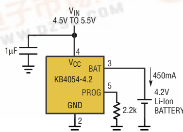
450mA Single Cell Li-Ion Charger
