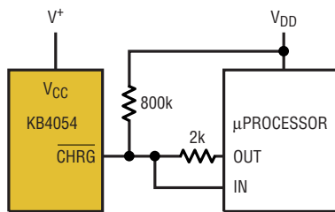
Figure 5. Using a Microprocessor to Determine \overline{\text{CHRG}} State
