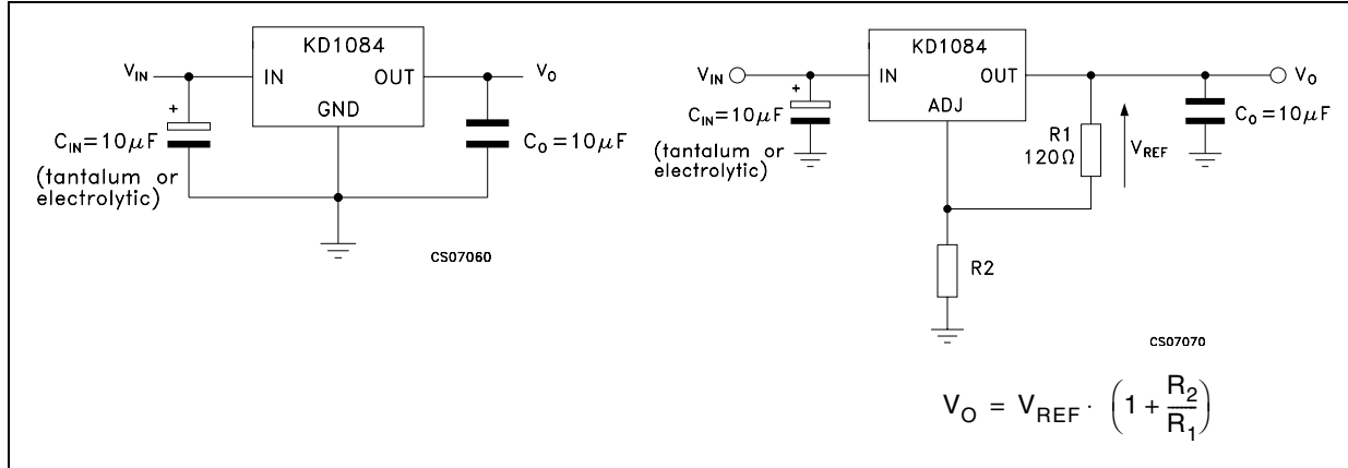
Figure 2. Application circuit
