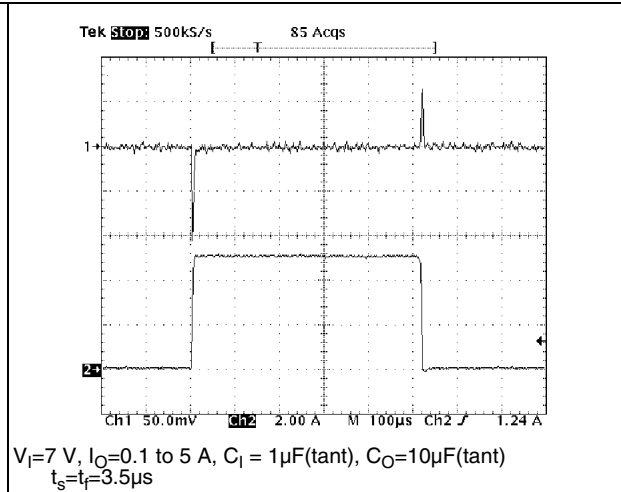
Figure 12. Load transient
