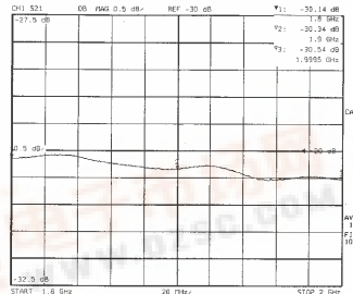
KEK-705H (COUPLING)
