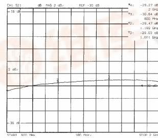
KEK-706H (COUPLING)
