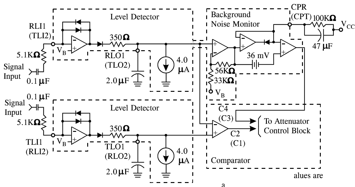
Figure 2. Level Detectors
