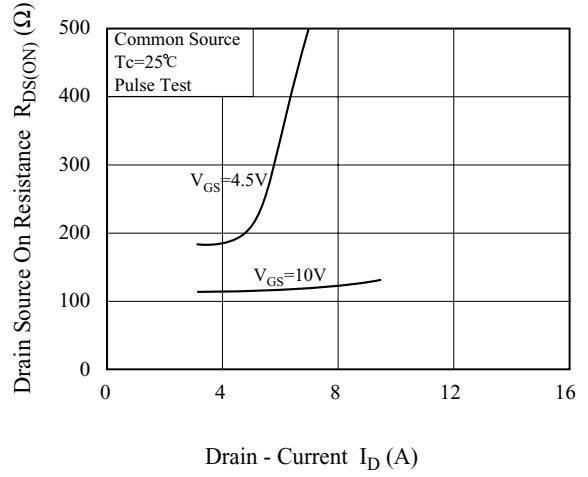
Fig2. R_{DS(ON)} - I_D
