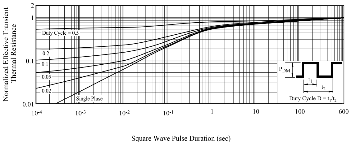
Fig10. Transient Thermal Response Curve
