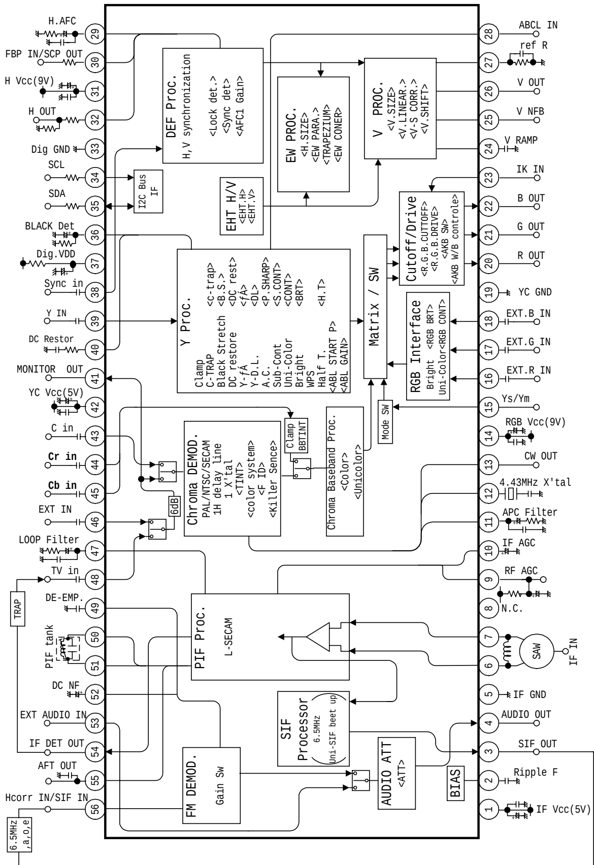
TB1254N BLOCK DIAGRAM
