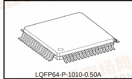
LQFP64-P-1010-0.50A
