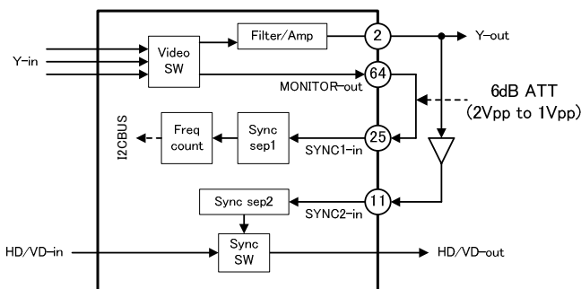
Fig. The signal route when A-SYNC = OFF
