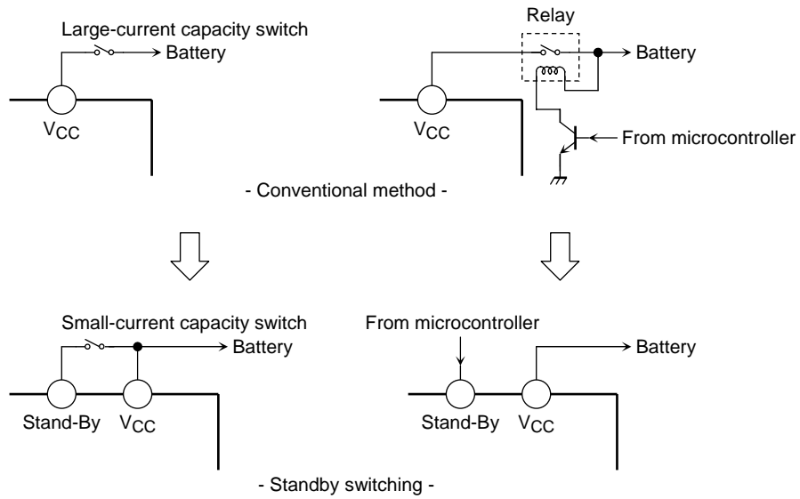
Figure 3 Standby switching
