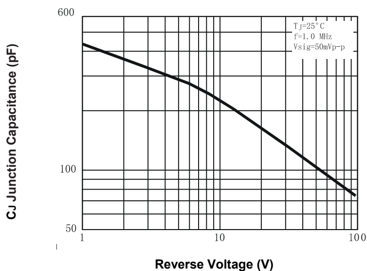
Fig.5-Typical junction capacitance
